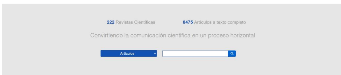
Figura 4. Buscador principal
